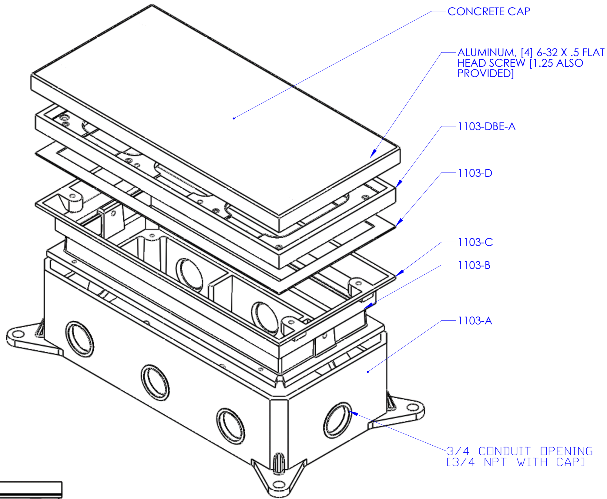
EXPLODED VIEW
