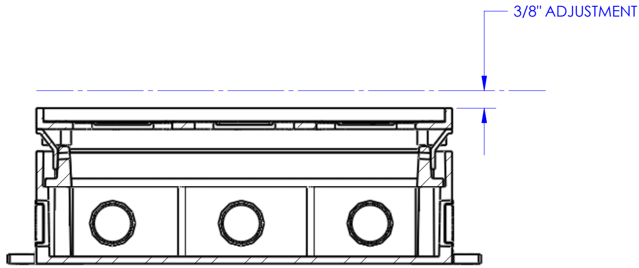
SECTION G-G
