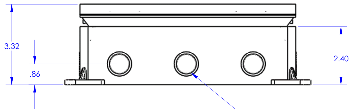
FRONT VIEW
