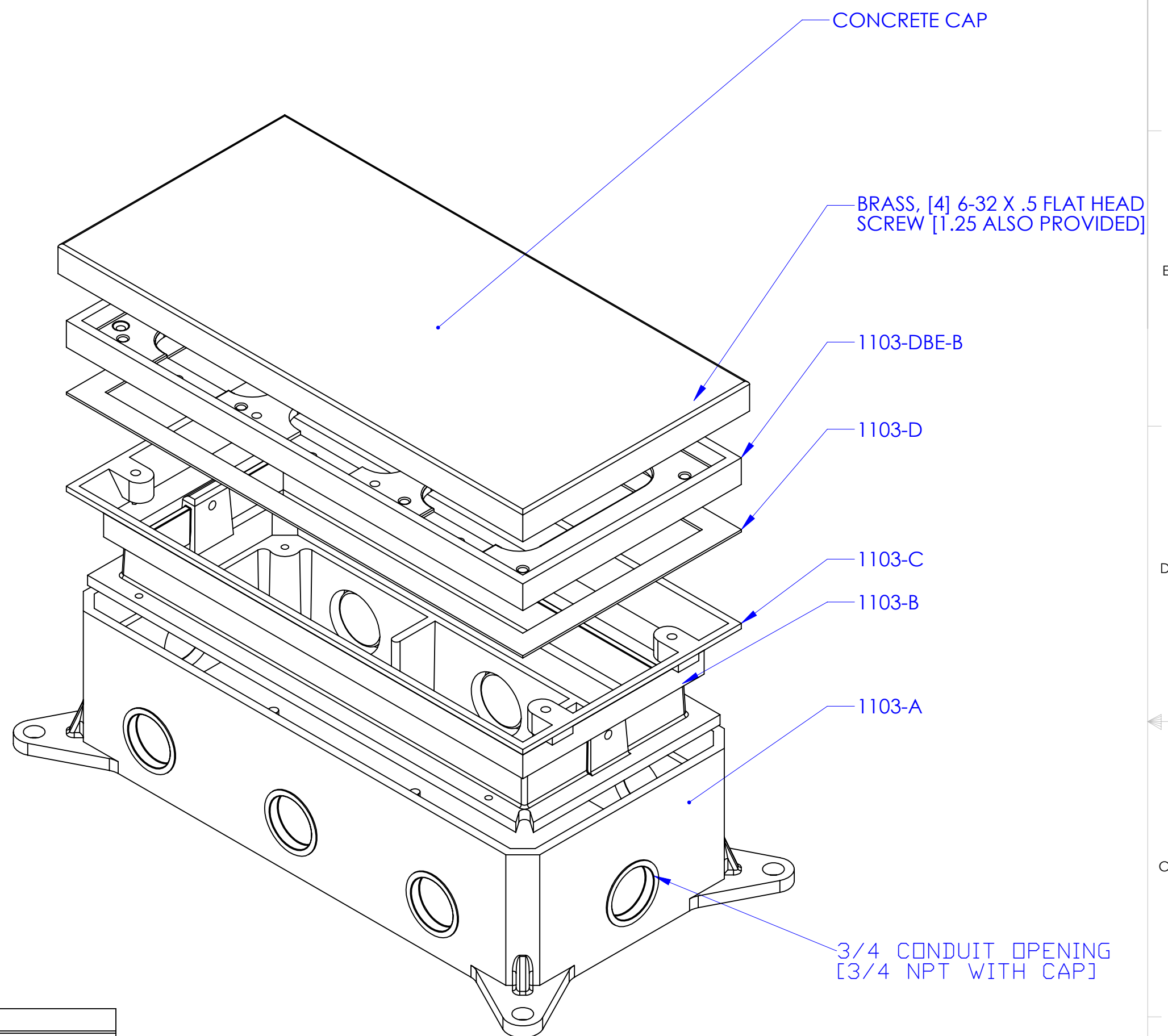
EXPLODED VIEW
