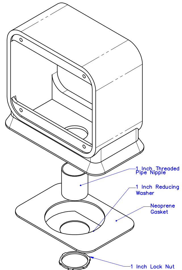
ISOMETRIC EXPLODED VIEW
