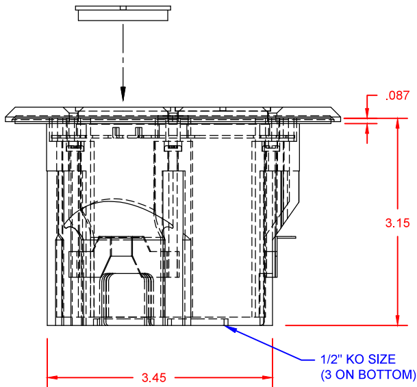
FRONT VIEW
