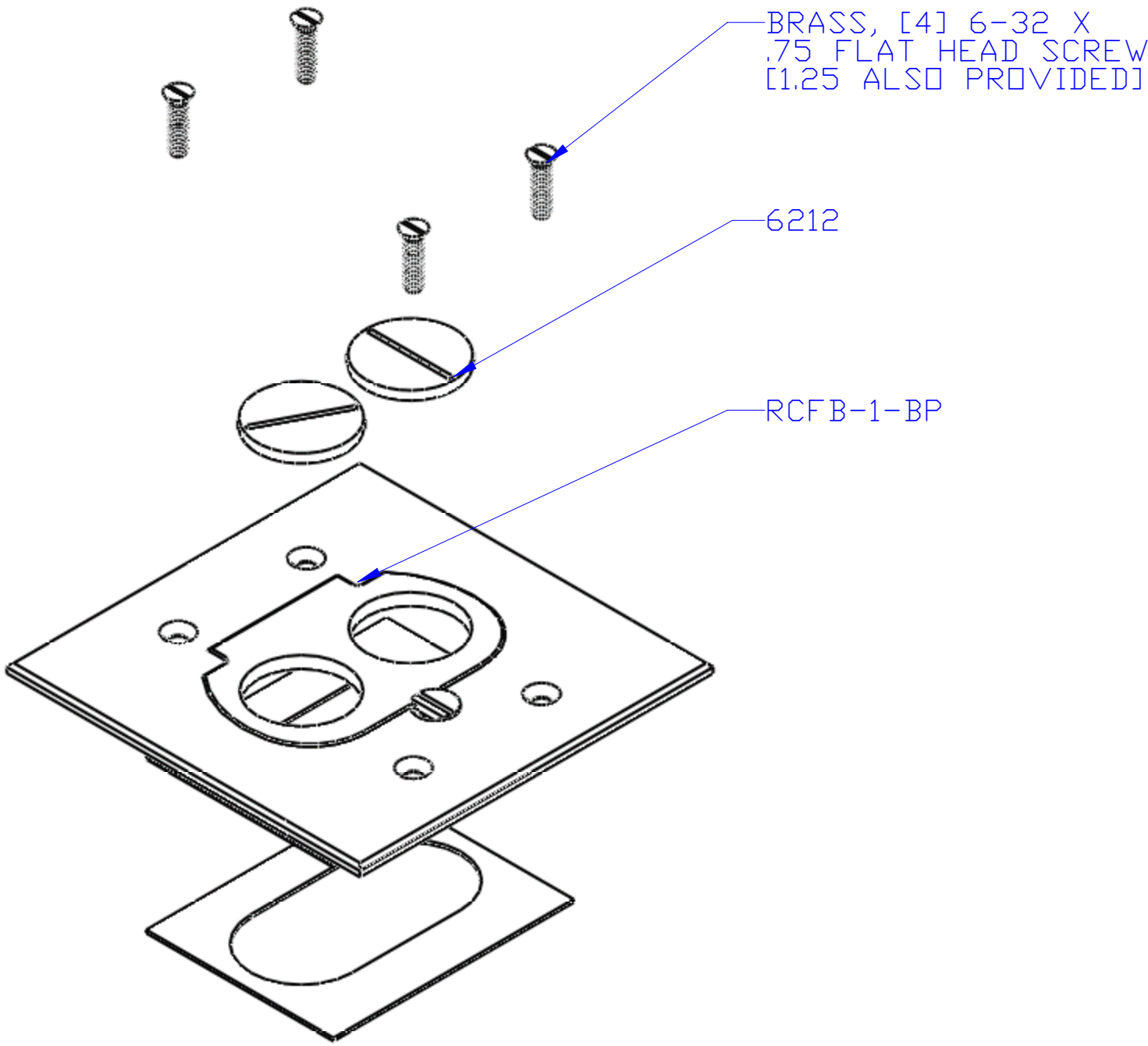
ISOMETRIC (EXPLODED) VIEW
