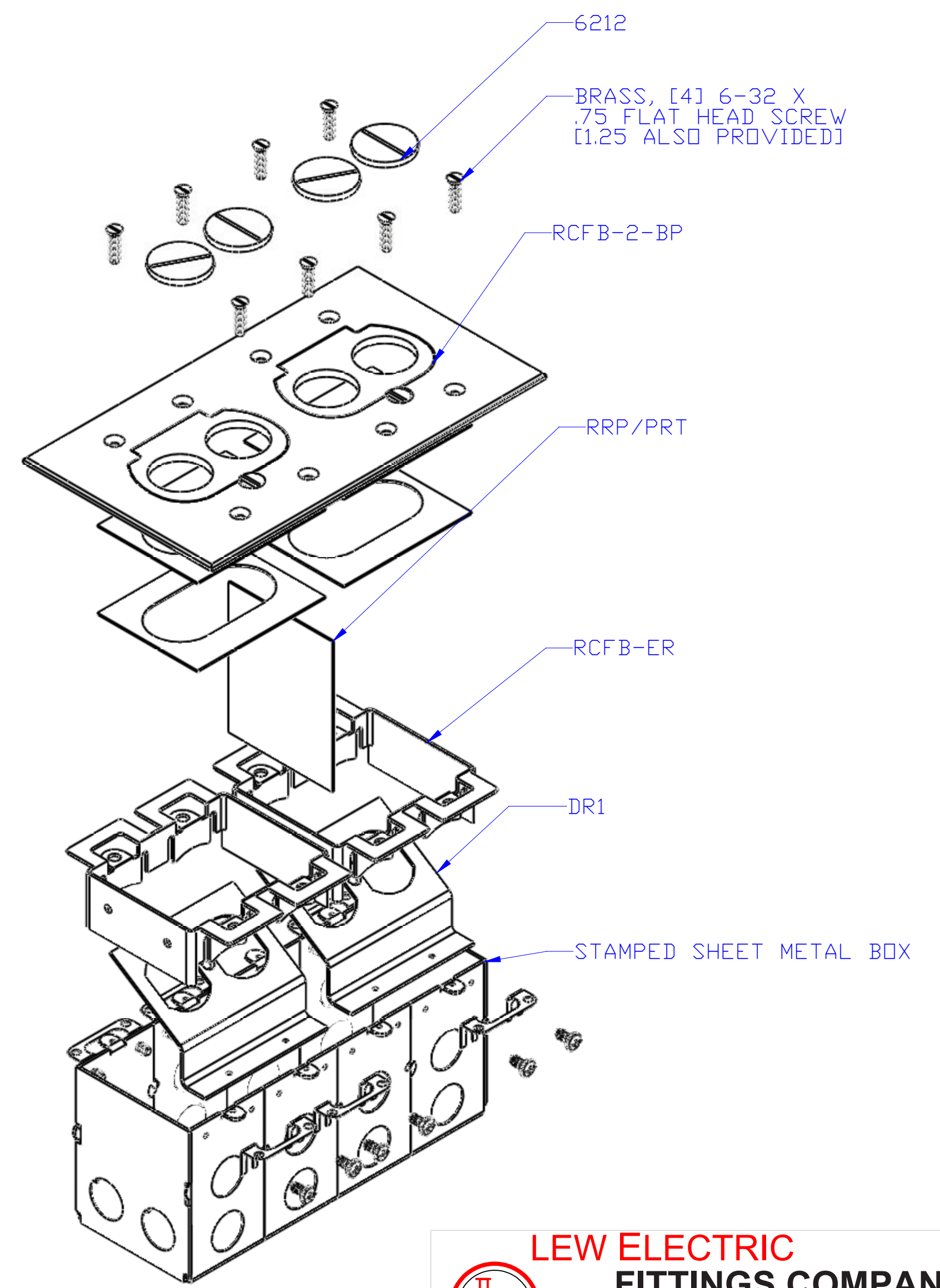
ISOMETRIC (EXPLODED) VIEW
