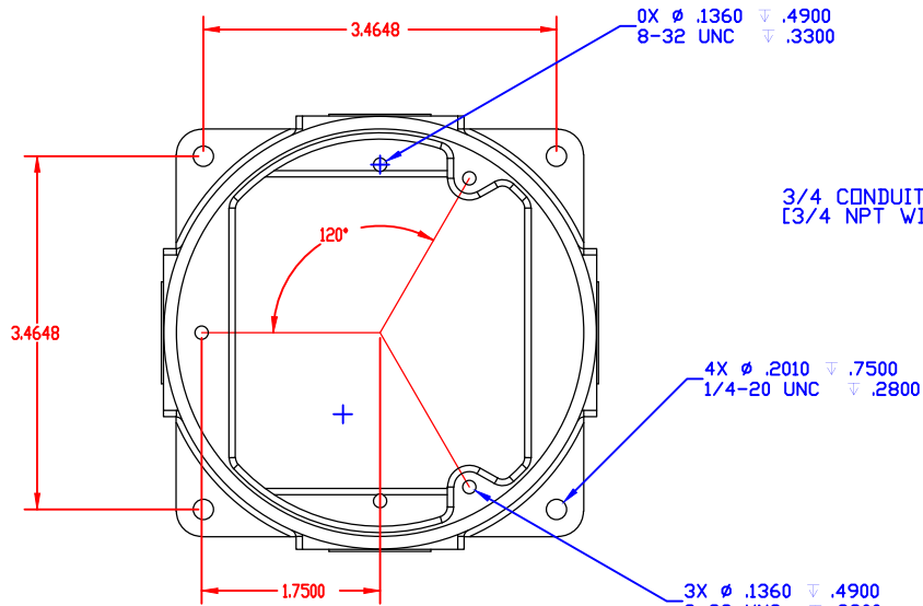
VIEW TOP
