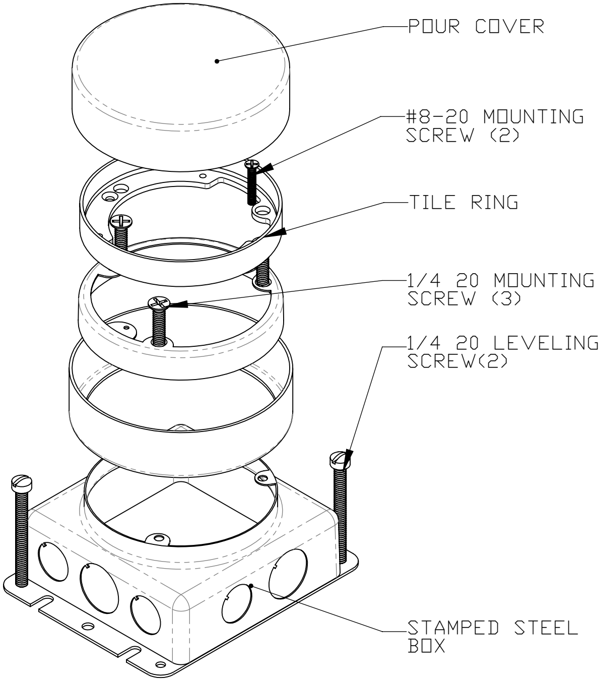
ISOMETRICE (EXPLODED)
