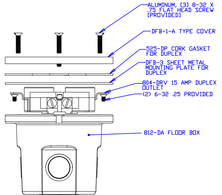
RIGHT [EXPLODED]
