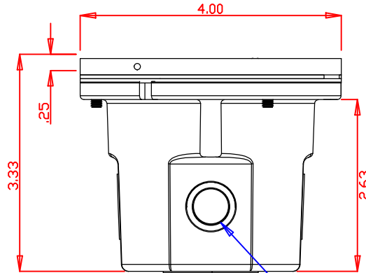
1/2 CONDUIT OPENING [1/2 NPT WITH CAP] OPPOSITE SIDE SAME
