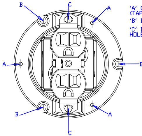
812 BOX W/D COVER
