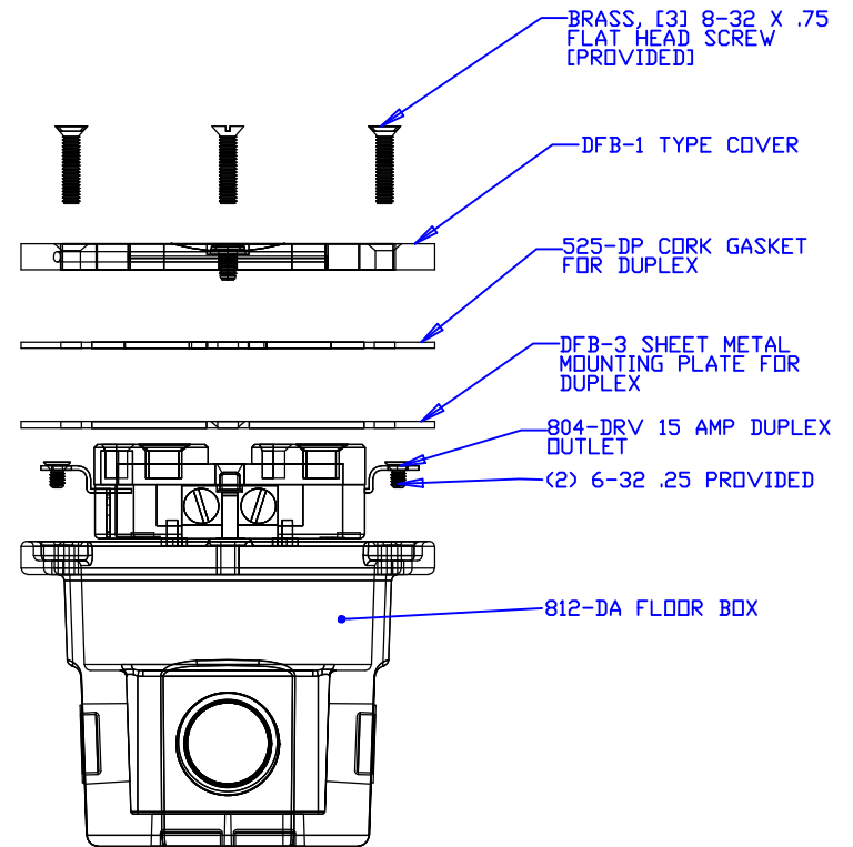
RIGHT (EXPLODED)
