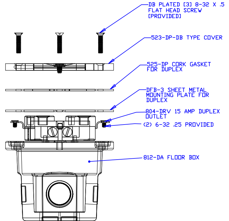
RIGHT (EXPLODED)
