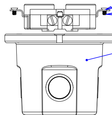
RIGHT [EXPLODED]
