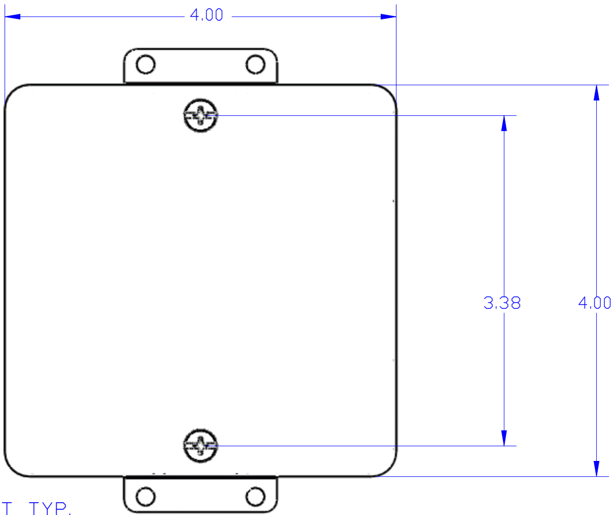
TOP VIEW
