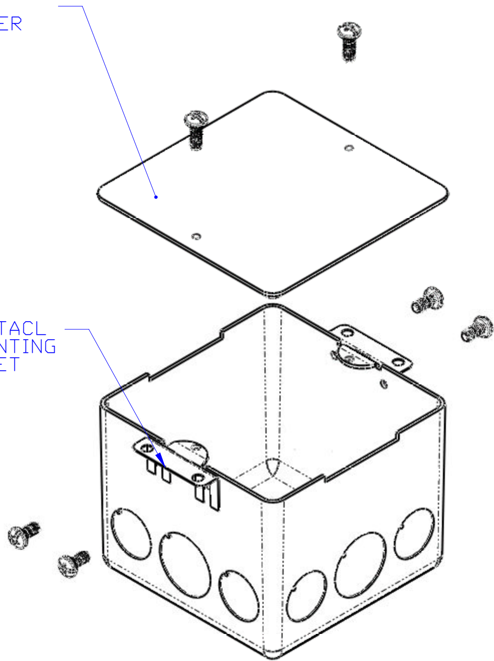
EXPLODED VIEW
