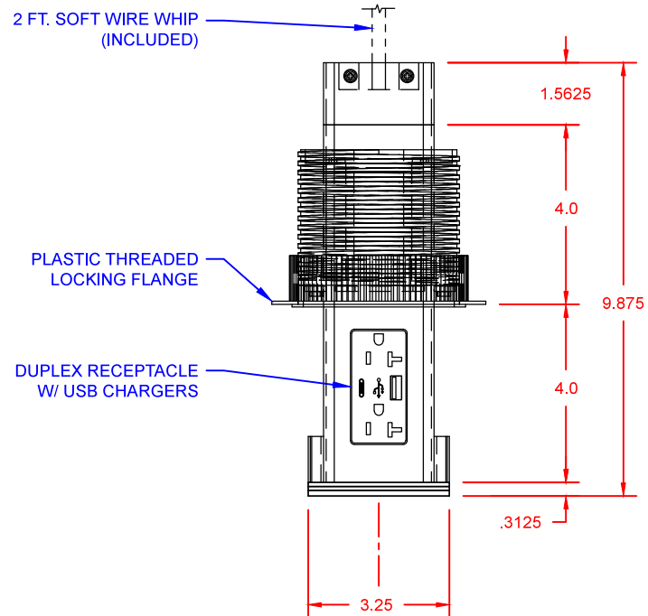
FRONT VIEW
